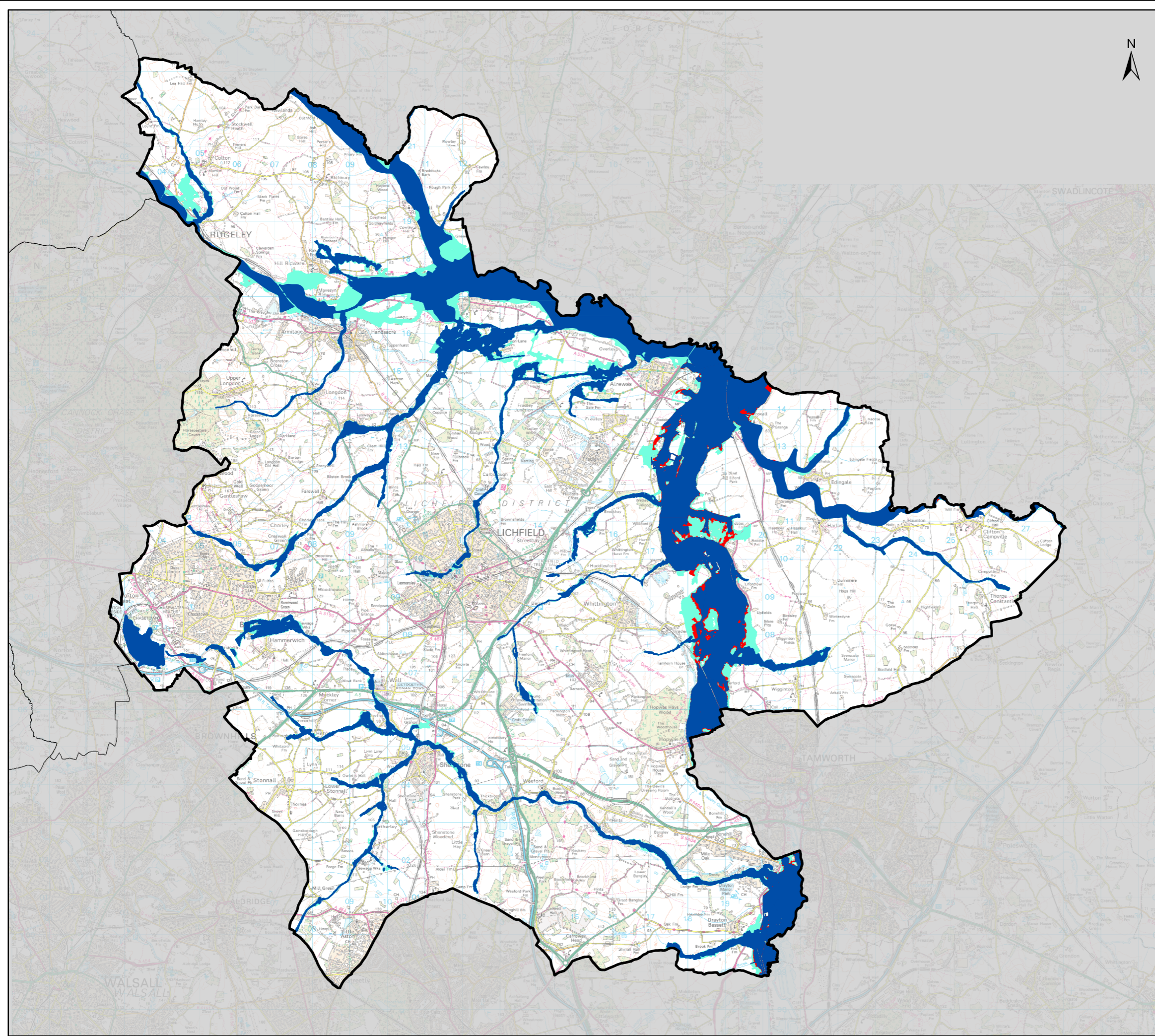
Figure FZ-LD Environment Agency Flood Zones in Lichfield District Council
