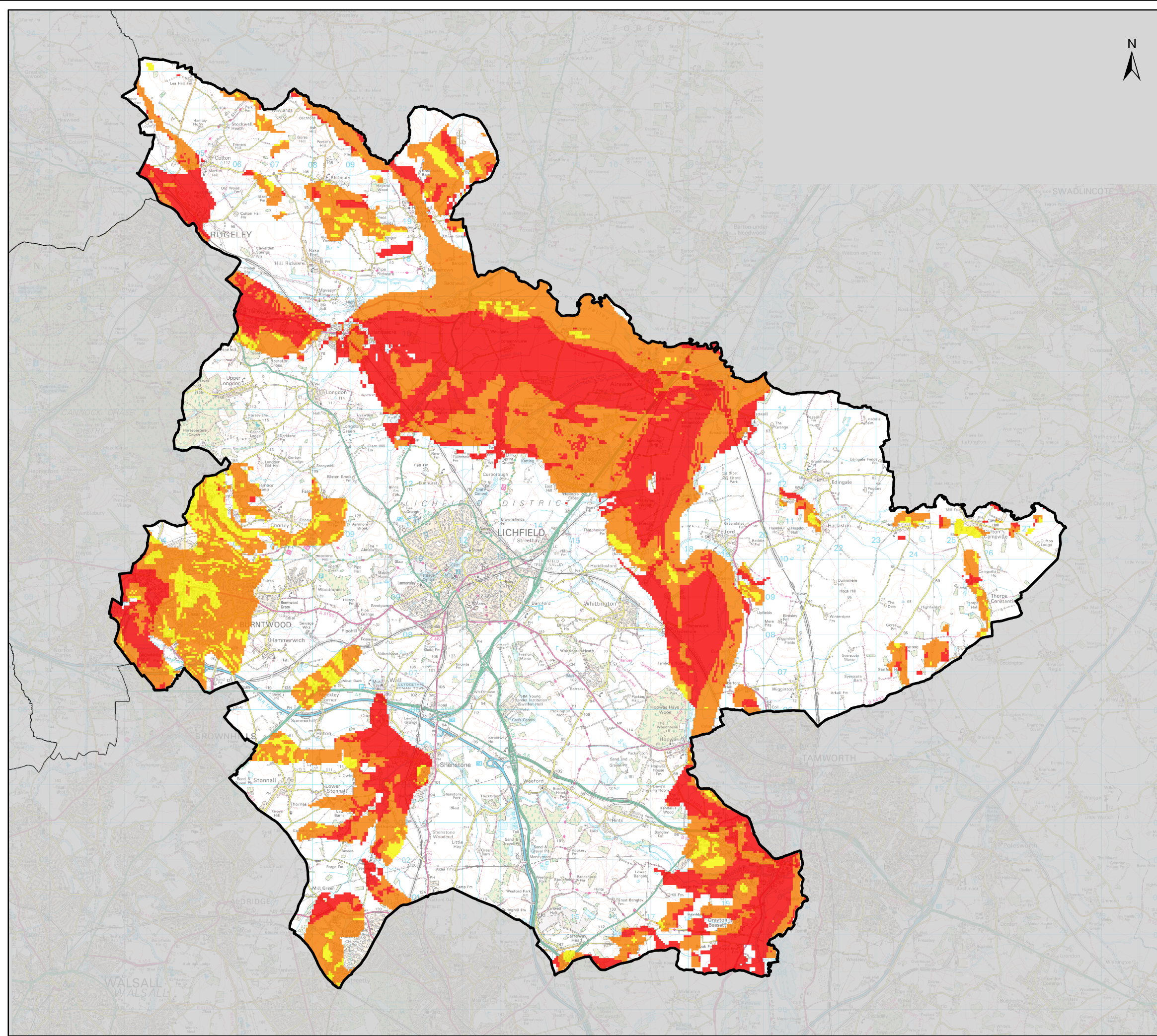
Figure SS1-LD Suitability of Infiltration SuDS techniques in Lichfield District Council
